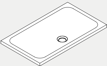
120×70×H4 cm RAPD12007040 Piatto doccia Rapid rettangolare 120×70 cm. 120×70 cm rectangular shower tray.
